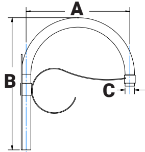
A 4 Wall Mount
