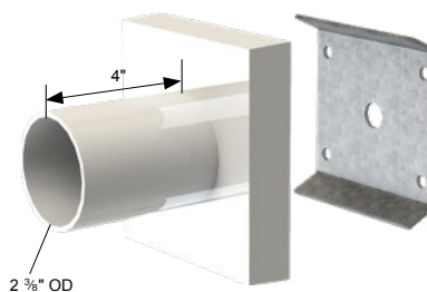
Wall Mount Slip Fit with 4" Arm WM-SFA
