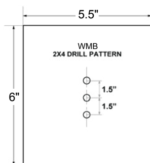
Wall Mount Bracket WMB
